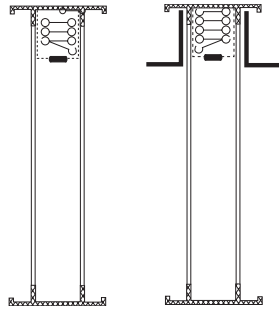
FD-VA FD-VB Vertical Type A Vertical Type B
