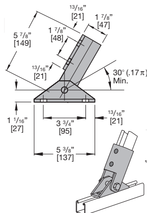
P2815 Adjustable Brace Fitting
