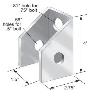
SAB SERIES Rigid Restraint Bracing
